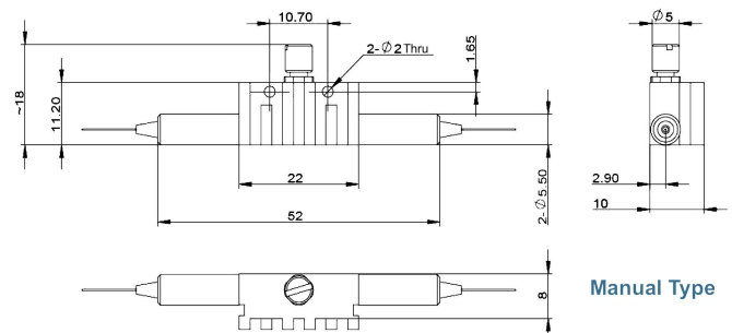
Screw Type
